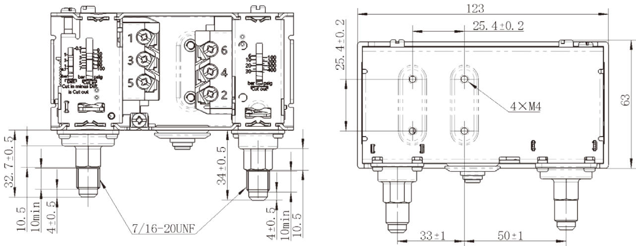
PSV15 × × L
