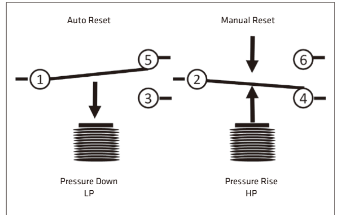
Dual PSV15AM
