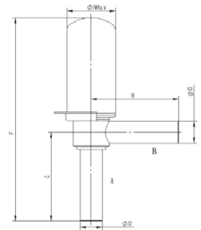
DPF (S03) 4.0~7.5
