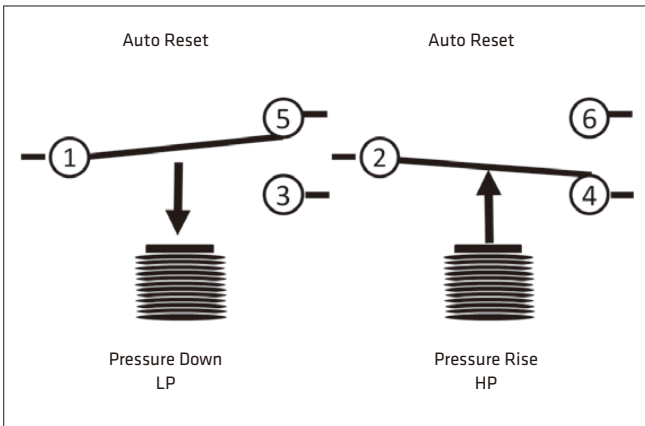
Dual PSV15AA
